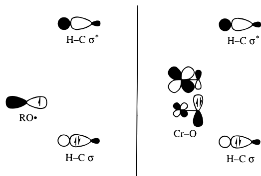
FIGURE 7. Frontier orbitals for hydrogen atom abstraction by alkoxy radicals (left) and a metal oxo complex (right). The vertical axis gives the approximate energy spacing. Reprinted from ref 20. Copyright 1995 American Chemical Society.
