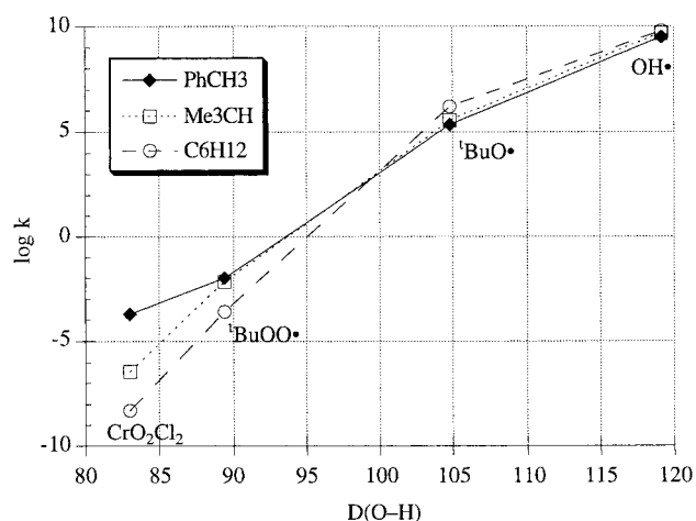
FIGURE 6. Rate constants for hydrogen atom abstraction vs the strength of the O–H bond formed, with D(\text{H}-\text{OCr}(\text{O})\text{Cl}_2) assumed to be 83 kcal/mol. Adapted from ref 20. 30
