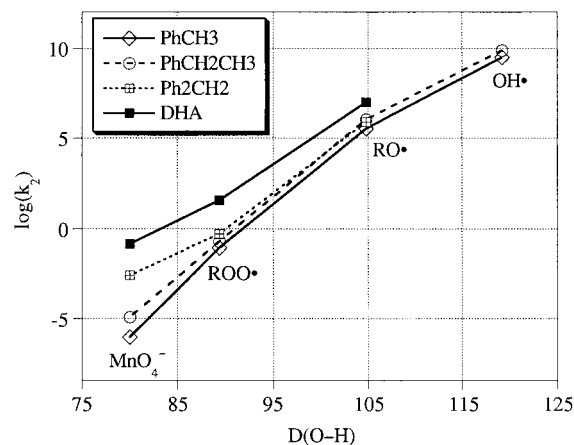
FIGURE 5. Rate constants for hydrogen atom abstraction by \text{HO}^\bullet , \text{RO}^\bullet , {}^t\text{BuOO}^\bullet , and \text{MnO}_4^- vs the strength of the O–H bond formed for toluene, ethylbenzene, diphenylmethane, and dihydroanthracene. Adapted from ref 35. 30
